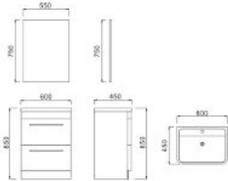
MC600F Vanity: 600 x 450 x 850mm Mirror: 550 x 750mm
