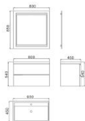
MF802 Vanity: 800 x 450 x 540mm Mirror: 800 x 850mm
