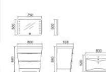
MP8002H Vanity: 800 x 520 x 840mm Mirror: 750 x 500mm
