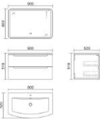
ST-900 Vanity: 900 x 520 x 518mm Mirror: 900 x 600mm
