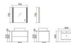
DW8002 Vanity: 800 x 520 x 518mm Mirror: 750 x 750mm
