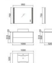
DW1002 Vanity: 1000 x 520 x 518mm Mirror: 950 x 750mm
