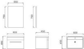
MC600W Vanity: 600 x 450 x 450mm Mirror: 550 x 750mm
