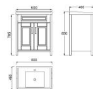
MW007B-N Vanity: 600 × 460 × 850mm Color: Ivory
