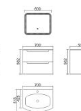
ST-700GV Vanity: 700 x 515 x 562mm Mirror: 600 x 500mm
