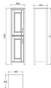
MW006A-N Vanity: 465 x 455 x 1782mm Color: Red oak
