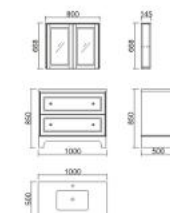
BR1002 Vanity: 1000 x 500 x 850mm Mirror: 800 x 145 x 668mm
