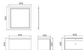
MF801 Vanity: 800 x 450 x 440mm Mirror: 800 x 850mm
