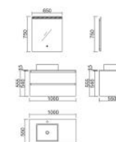
DW1000 Vanity: 1000 x 550 x 555mm Mirror: 650 x 750mm
