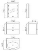
ST-700 Vanity: 700 x 515 x 562mm Mirror: 750 x 600mm
