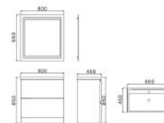
MF802F Vanity: 800 x 450 x 850mm Mirror: 800 x 850mm
