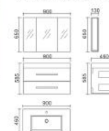
JS036 Cabinet: 900 x 460 x 585mm Mirror: 900 x 130 x 650mm
