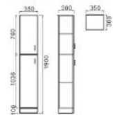
CG30D(G) Cabinet: 350 x 300 x 1900mm
