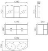
ST-1200 Vanity: 1220 x 550 x 562mm Mirror: 700 x 1200 x 120mm
