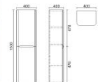
BN4002SS Cabinet: 400 x 300 x 1500mm
