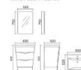
MY6502 Vanity: 650 x 520 x 840mm Mirror: 500 x 750mm
