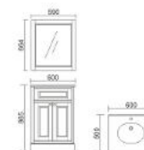
TL600 Vanity: 600 x 500 x 865mm Mirror: 590 x 664mm
