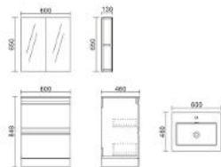
ZRF6002GR Vanity: 600 x 460 x 848mm Mirror: 600 x 130 x 650mm
