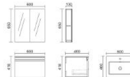
ZRW6001WH Vanity: 600 x 460 x 418mm Mirror: 600 x 130 x 650mm
