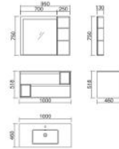
HP1002 Vanity: 1000 x 460 x 518mm Mirror: 700 x 130 x 750mm Side cabinet: 250 x 130 x 750mm
