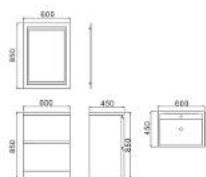
MF602F Vanity: 600 x 450 x 850mm Mirror: 600 x 850mm
