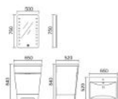
MP6501H Vanity: 650 x 520 x 840mm Mirror: 500 x 750mm
