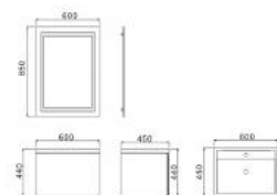
MF601 Vanity: 600 x 450 x 440mm Mirror: 600 x 850mm
