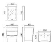
MP6502G Vanity: 650 x 520 x 840mm Mirror: 500 x 750mm
