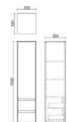
AG1500D-40SS Cabinet: 350 x 360 x 1500mm
