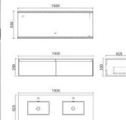
AG1500D Vanity: 1500 x 525 x 350mm Mirror: 1500 x 550mm
