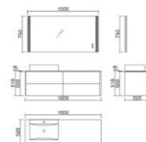
DW1604 Vanity: 1600 x 520 x 518mm Mirror: 1500 x 750mm
