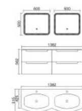
ST-1380GV Vanity: 1382 x 515 x 562mm Mirror: 600 x 500mm
