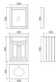
SK65 Cabinet: 650 x 500 x 835mm Mirror: 600 x 700mm
