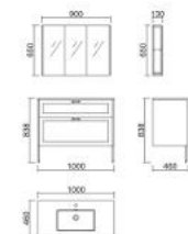
TP1002 Vanity: 1000 x 460 x 838mm Mirror: 900 x 130 x 650mm
