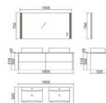
DW1604D Vanity: 1600 x 520 x 518mm Mirror: 1500 x 750mm
