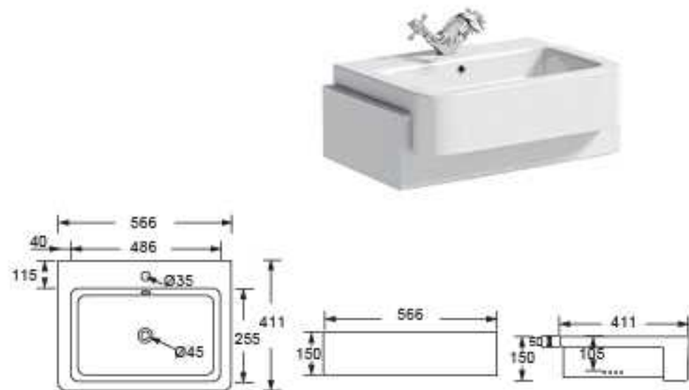
LB6100 Semi recessed countertop basin Size:566×411×150mm
