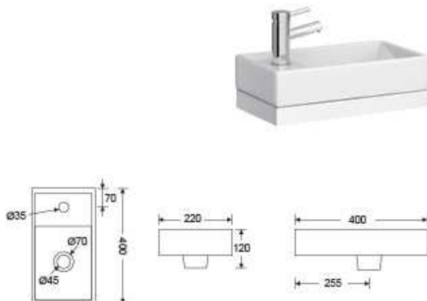
LB5400 Vanity cloakroom basin Size:400×220×120mm
