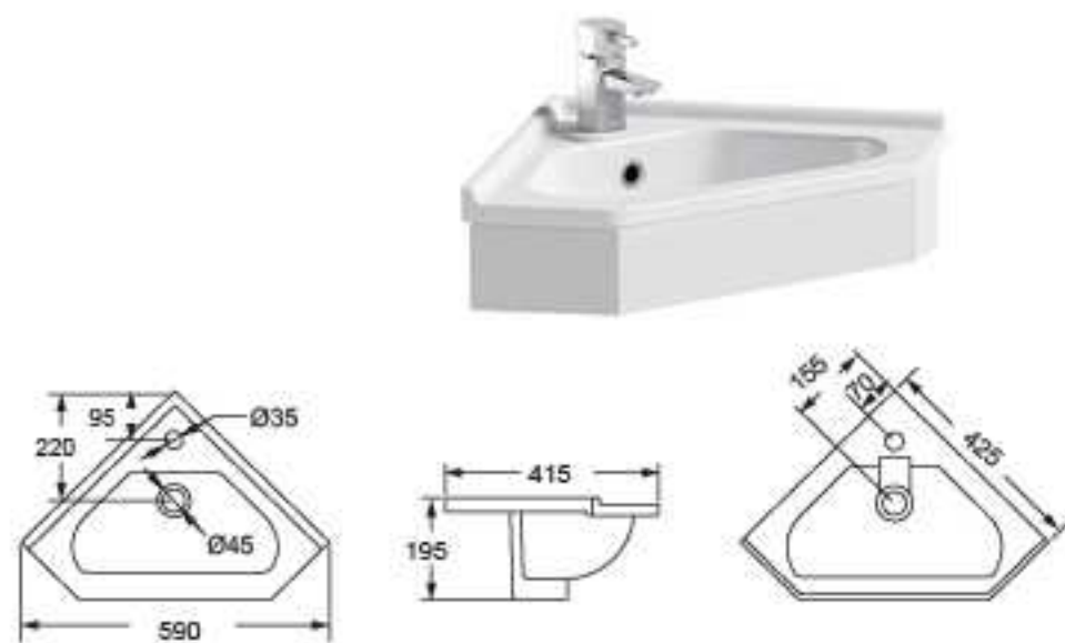
LB8200 Vanity corner countertop basin Size:590×415×195mm
