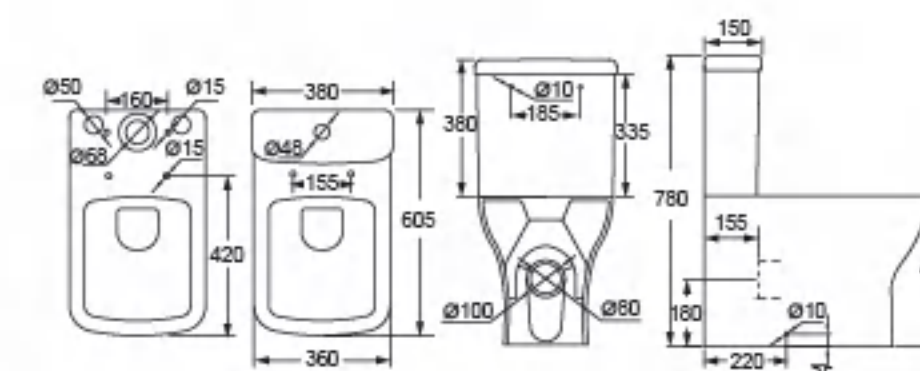
CT8801FHA Comfort Height
